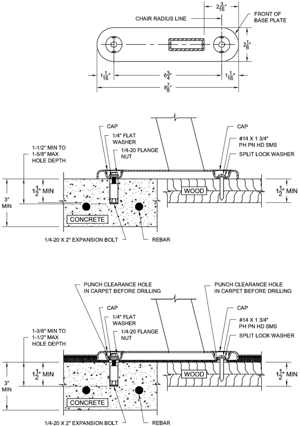
Figure 5 - Lyric – Floor Mounting Details
